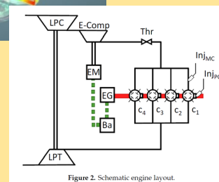
Figure 2. Schematic engine layout.
